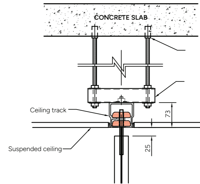
Head Track Fixing Detail
