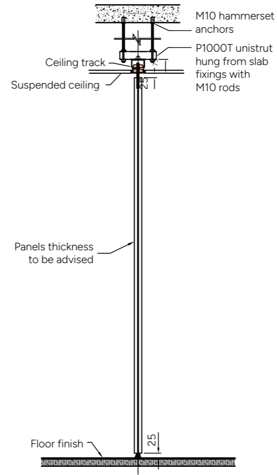
Vertical Section of Panel & Track Fixing
